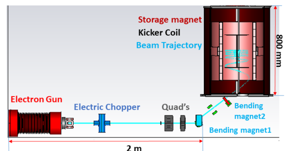
Figure 1: The side view of the 3D model of Spiral Injection test Experiment.
