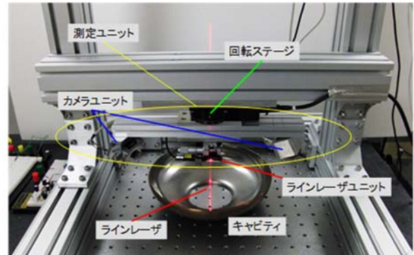
Figure 4 Measuring system
