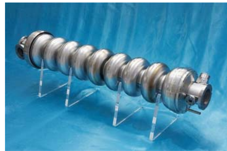
Figure 1 Accelerating cavity
