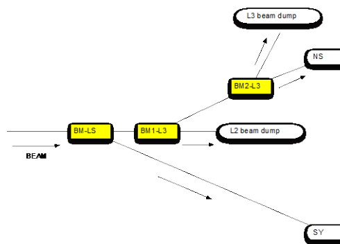
Figure 3: Beam routes from SPring-8 linac.
