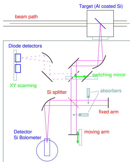
Figure 2: Setup of the CTR measurement.
