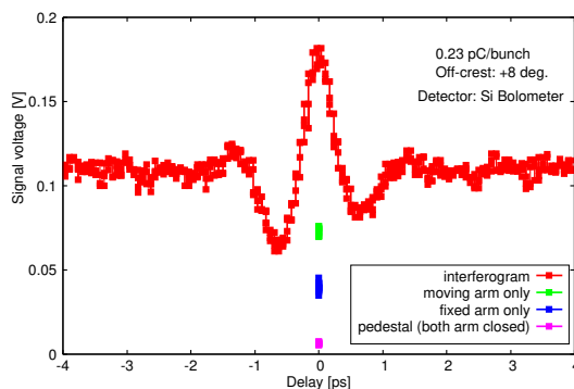
Figure 5: Interferogram of the Michelson interferometer.
