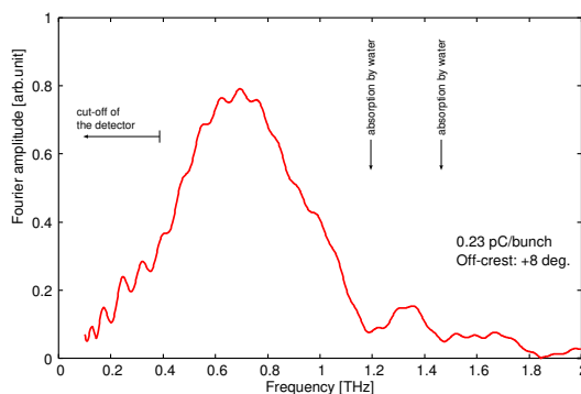
Figure 6: Fourier spectrum obtained from the CTR interferogram.
