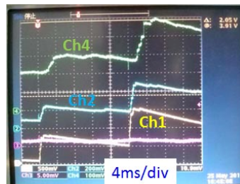
Figure 4: Acoustic signals from AC_34_4. The sensor locations are Ch1=input coupler, Ch2=input wave guide and Ch3=output coupler.
