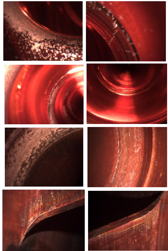
Figure 8: Observations of #63 seen by a borescope inserted from the wave guide into a coupler cell and viewing four directions from the coupler cell. Lined up from top to bottom are first iris, second iris, beam pipe iris and wave guide iris lip. Left figures are those of input coupler side and right of output coupler side.
