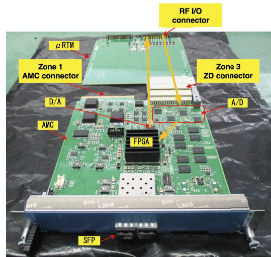
Figure 4: Pictures of the longitudinal mode-by-mode feedback processor. [7]
