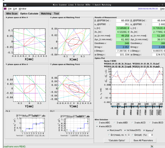
Figure 7: Wire scan measurement of electron beam at linac 5 sector.
