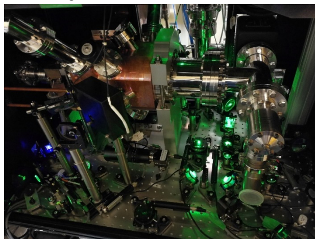
Figure 5: Optics system inside the RF box.
