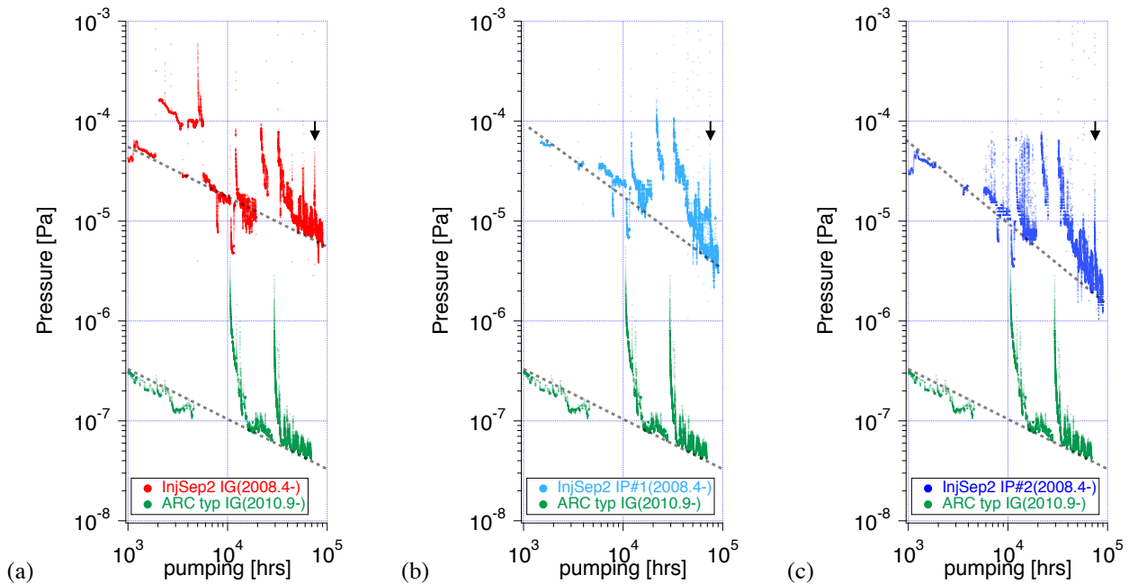
Figure 4: Pumping curve of a) IG, b) IP#1, and c) IP#2 of the chamber of injection septum II and a typical position in ARC. Arrows indicate the time when the pump was changed at 2016.9. The start time of ARC data was set as 2010.9 when the pump was installed in this place. The slopes of dashed lines are a) -0.5(both IG and ARC), b) -0.73, c) -0.81.
