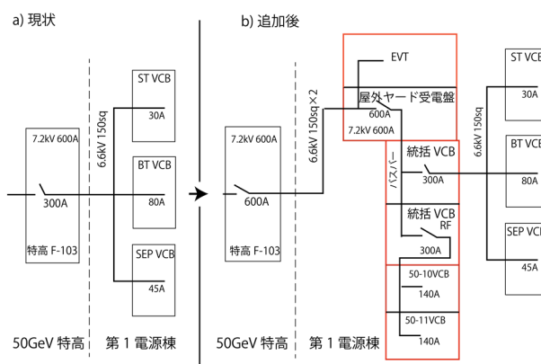
Figure 3: Power system diagram of the F-103.
