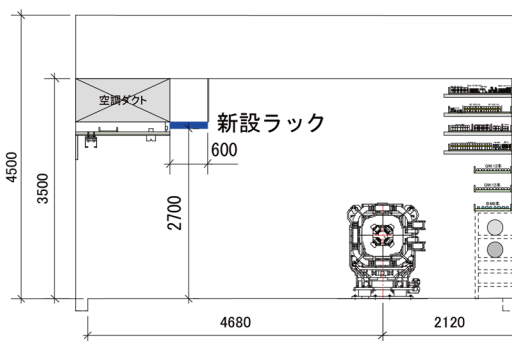
Figure 5: Cross-sectional view of the Ins-A.
