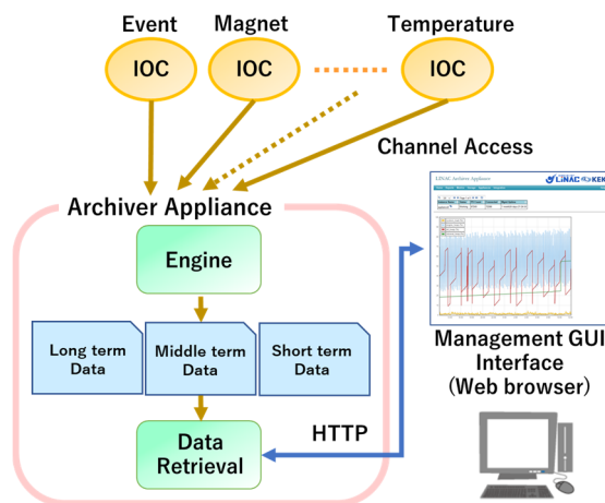
Figure 4: Schematic view of Archiver Appliance of the KEK injector linac.
