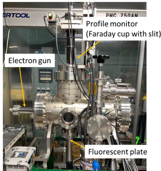
Figure 2: Off-line test stand for electron beam measurement.
