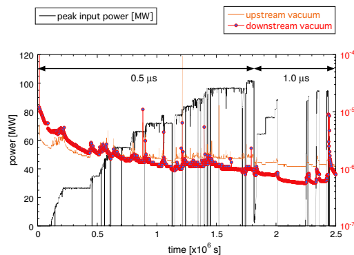
Figure 5: Conditioning history of the S-band accelerating structure #002.
