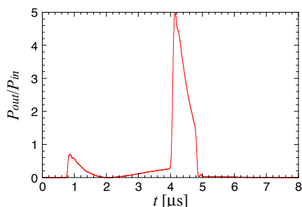
Figure 2: Waveform of an output power of the KEK RF pulse compressor. P_{out}/P_{in} shows the power multiplication factor.
