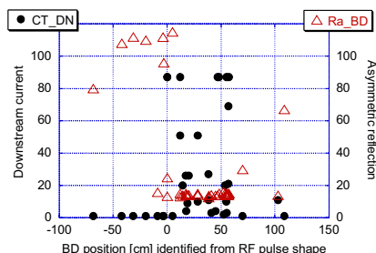
Breakdowns around ACC Structure
