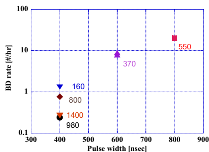
Breakdown Rate at 50Hz and normalized to 65MV/m
